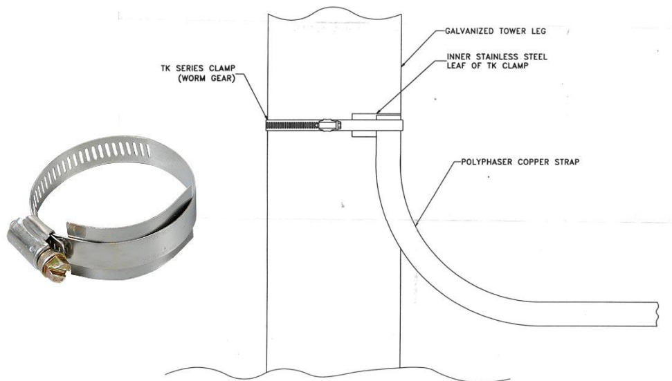
Figure 3 - TK Series Clamp Transition from Tower Leg to Copper Strap
