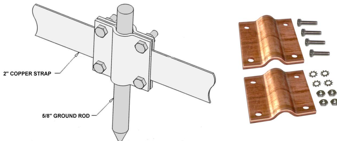
Figure 19 - DXE-58R-112S Ground Rod to Copper Strap Bonding Clamp
