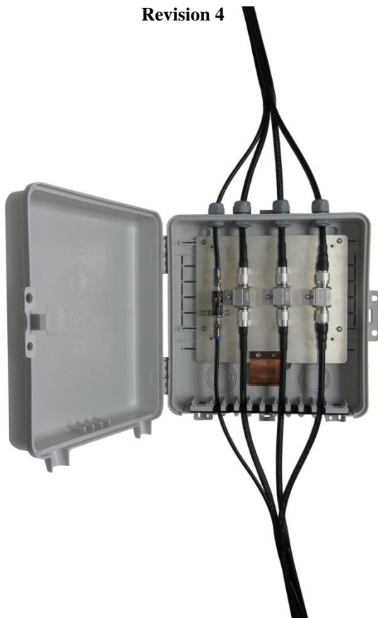
DXE-UE-2P shown with optional lightning protection devices installed
