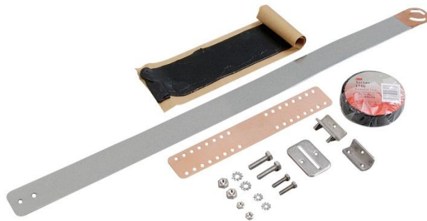
Figure 6 - PPR-UNI-KIT-2CT for Copper Shield to Galvanized or Aluminum Towers
