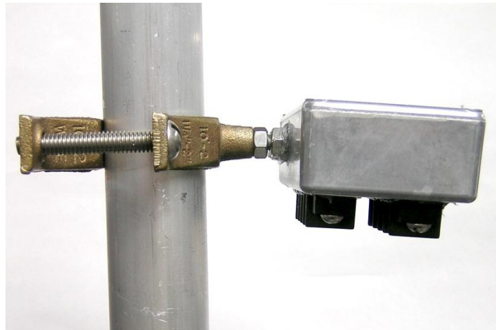
Figure 15 - PPR-IS-RCT Mounted to Tower Leg using a PPR-J-2 Clamp.
