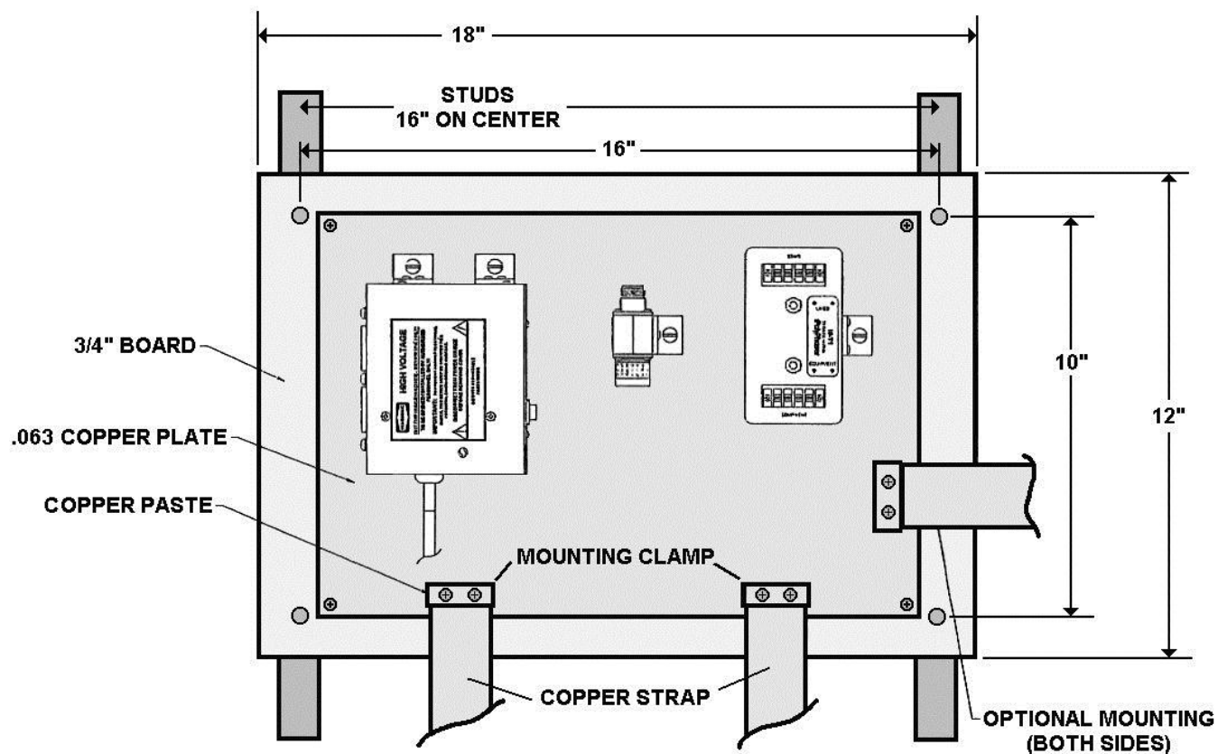
Figure 23 - Single Point Ground Panel with Optional Protectors Mounted
