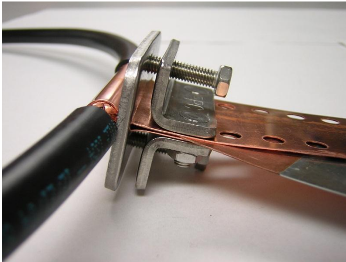
Figure 12 - Completed Strap Assembly.
