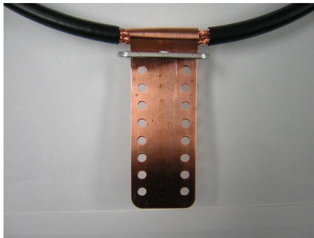
Figure 8 - Strap Wrapped Around the Shield with Bracket In-Place
