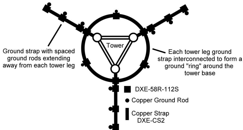
Figure 4: Top View of a Tower Ground System
