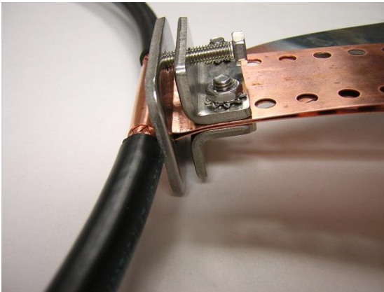
Figure 9 A & B - Grounding clamp assembly ready to be tightened.
