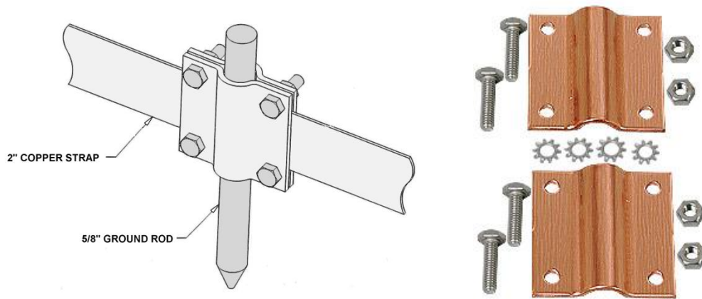
Figure 2: DXE-58R-112S Ground Rod to Strap Clamp
