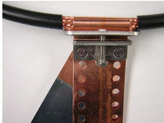
Figure 9 A & B - Grounding clamp assembly ready to be tightened.
