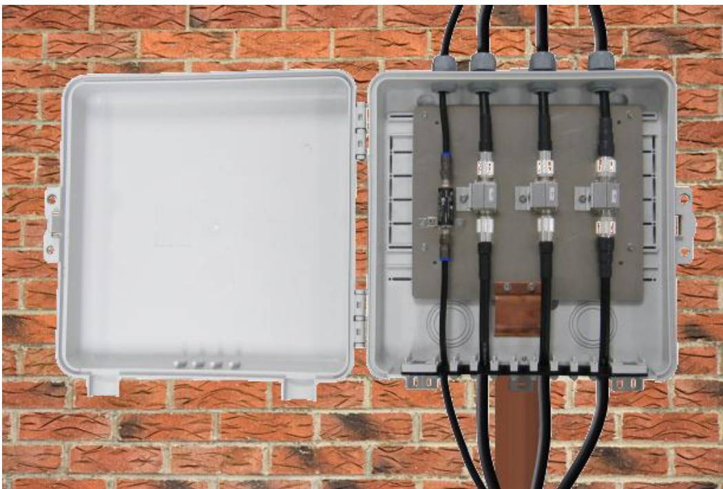
Figure 18 - The DXE-UE-2P Weathertight Enclosure (Shown with Optional Equipment Mounted)
