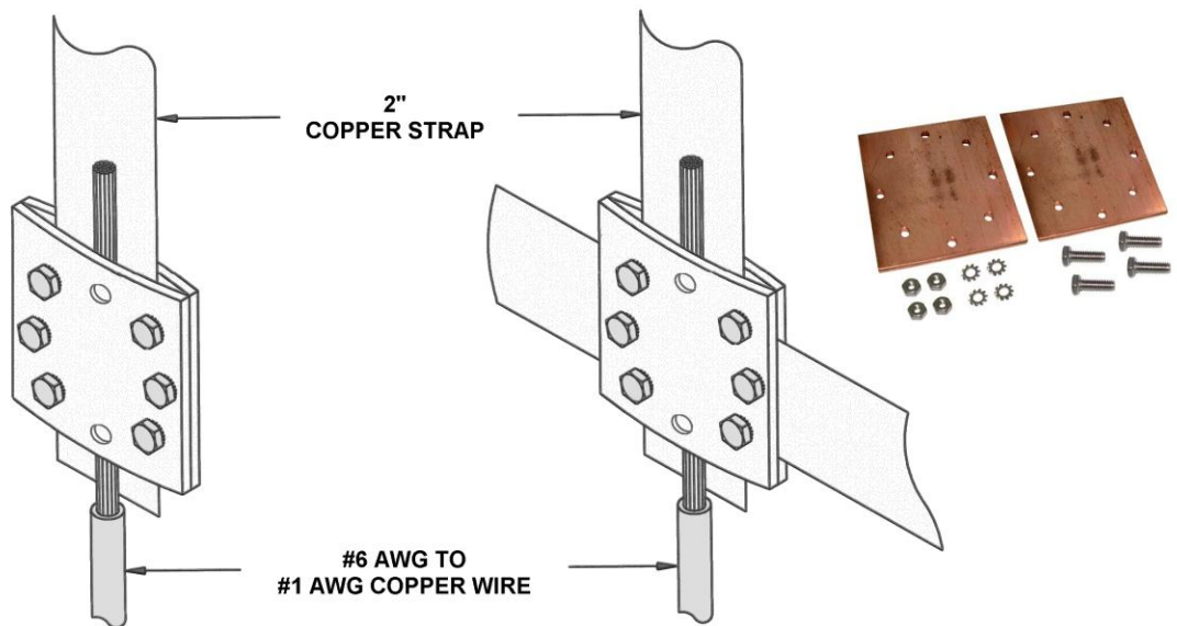
Figure 5 - DXE-MSC-3 Copper Strap Bonding Clamp
