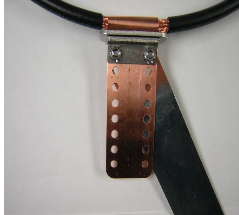
Figure 11- Bolts fit to inside of the dimple
