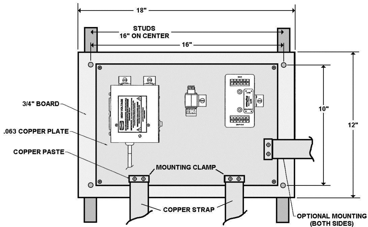
Figure 16 - DXE-CU-SPGP (shown with optional protectors)
